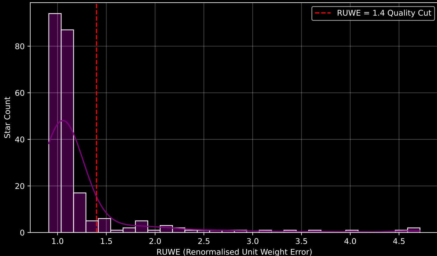
GALAH DR4 Field [9217] RUWE Distribution (n= 235)
