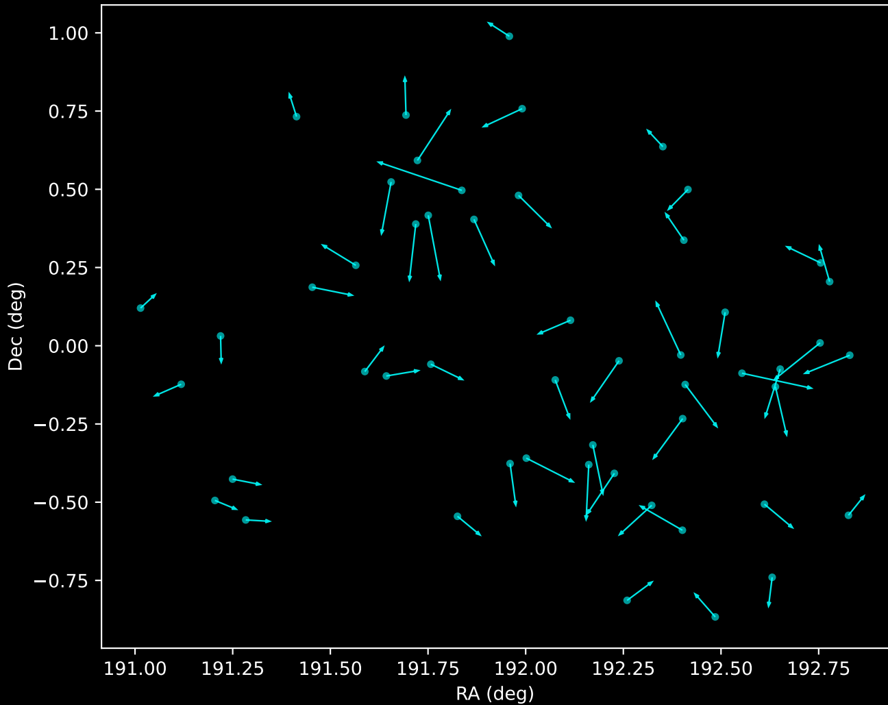
GALAH DR4 Noise Stream Proper Motion Vectors (n=52)
