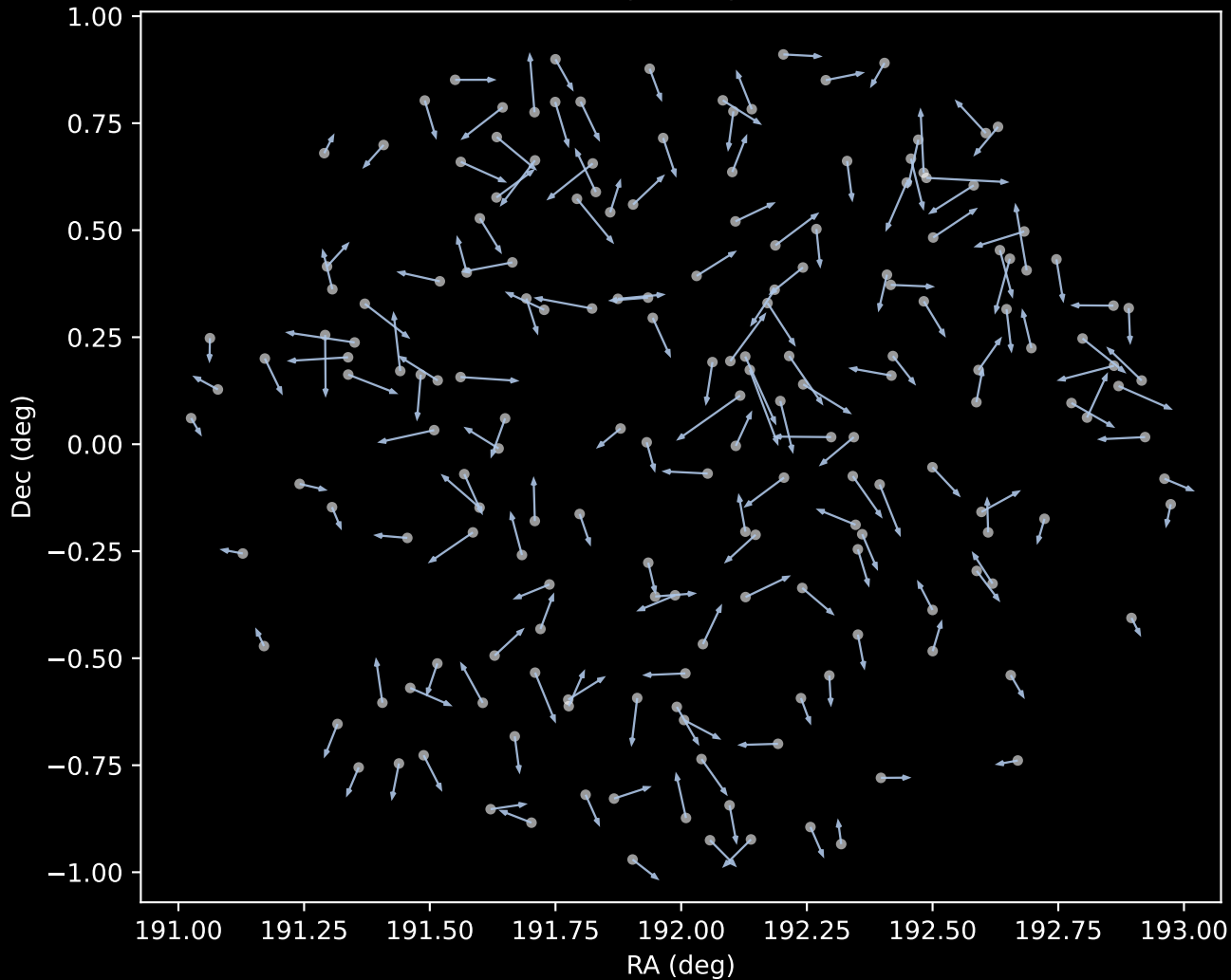
GALAH DR4 Cluster 1 Proper Motion Vectors (n=183)
