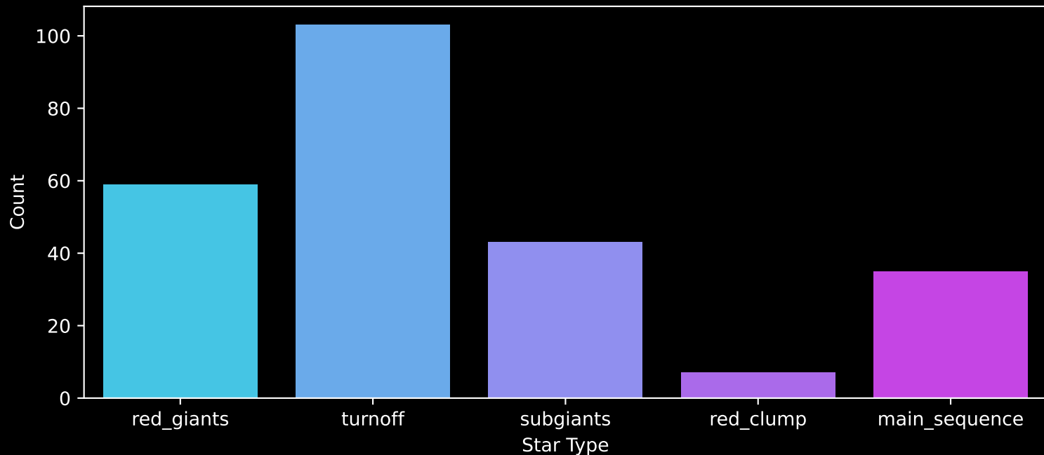
GALAH DR4 Field: [9217] Count plot of Star Type
